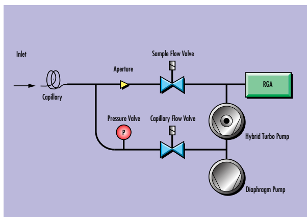
QMS schematic
